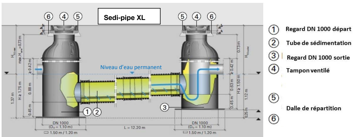
Figure 2 : Sedi-pipe XL
