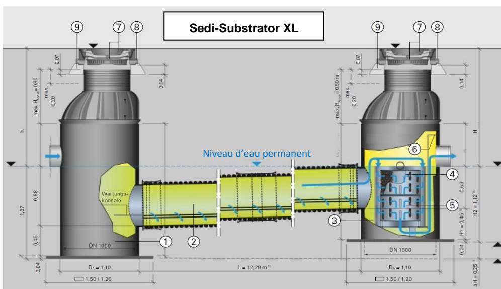
Figure 5: Sedisubstrator XL
