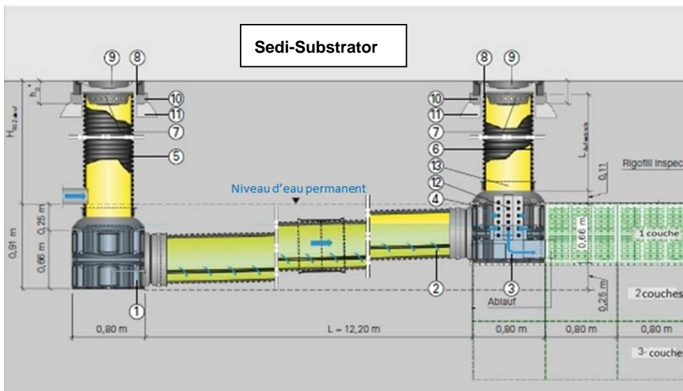
Figure 4 : Sedisubstrator
