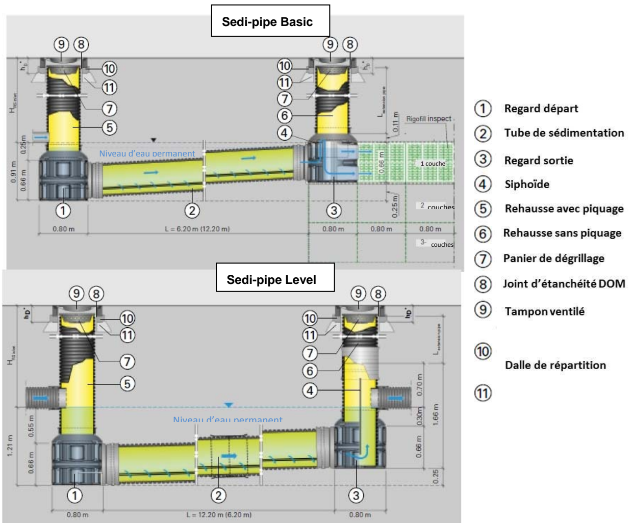
Figure 1a et 1b: Sedi-pipe basic & Level
